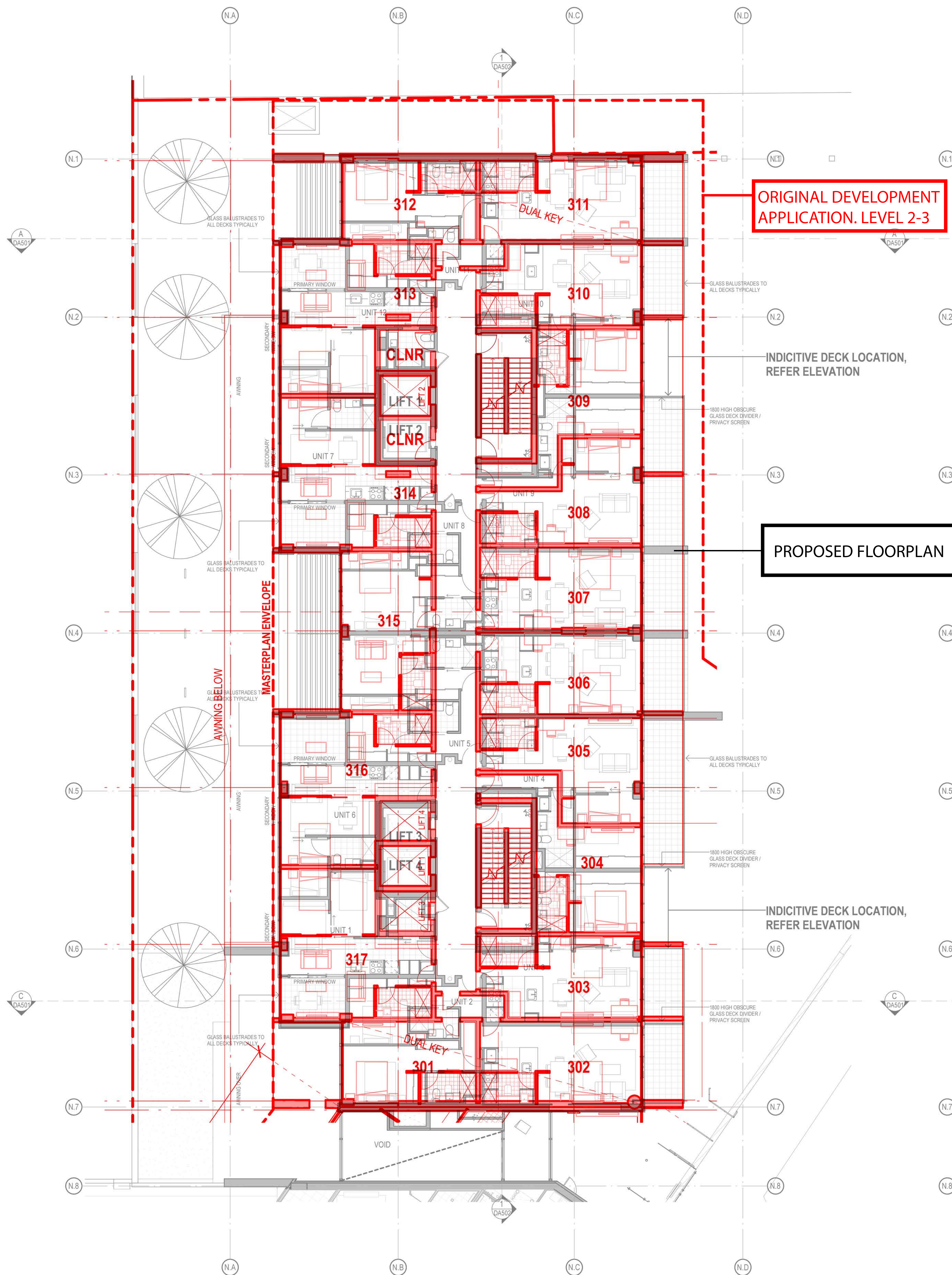
1 LEVEL 01-06 NORTH PLAN 1:100
